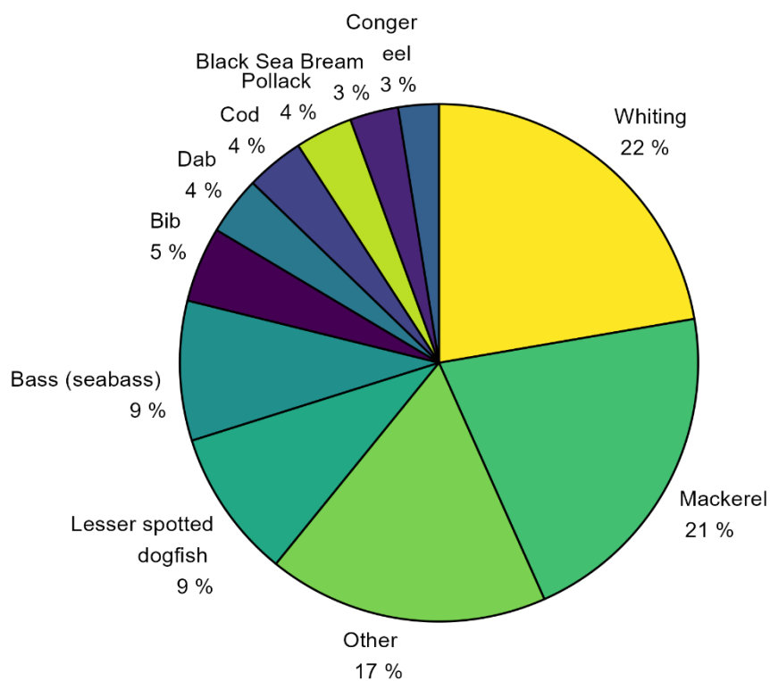
Figure 43. Catch composition by number for the UK in 2021 for multilevel regression and poststratification (MRP) (A) and reweighting (B) with the top 10 most commonly caught fish displayed.
