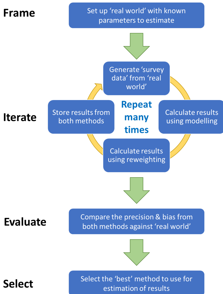
Figure 4. Simulation study approach used to assess the 'best' method for estimating numbers of anglers and catches.
