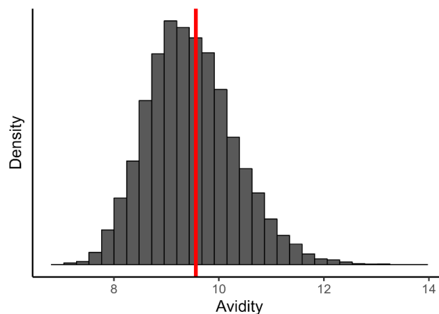
Figure 20. A posterior predictive check of the number of days fished (avidity) by UK sea anglers. The bars show the proportion of each value from the posterior distribution of the fitted Bayesian model and the red line shows the estimate from the data.
