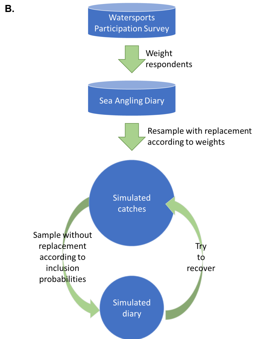
Figure 5. Schematic showing the simulation approaches to assess the robustness of the reweighting and model-based estimation methods for the effort (A) and catch (B).
